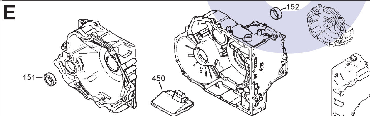
CASE, FILTER & VALVE BODY COVER
