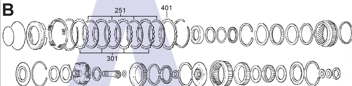
LOW & REVERSE BRAKE & FRONT & REAR PLANETS
