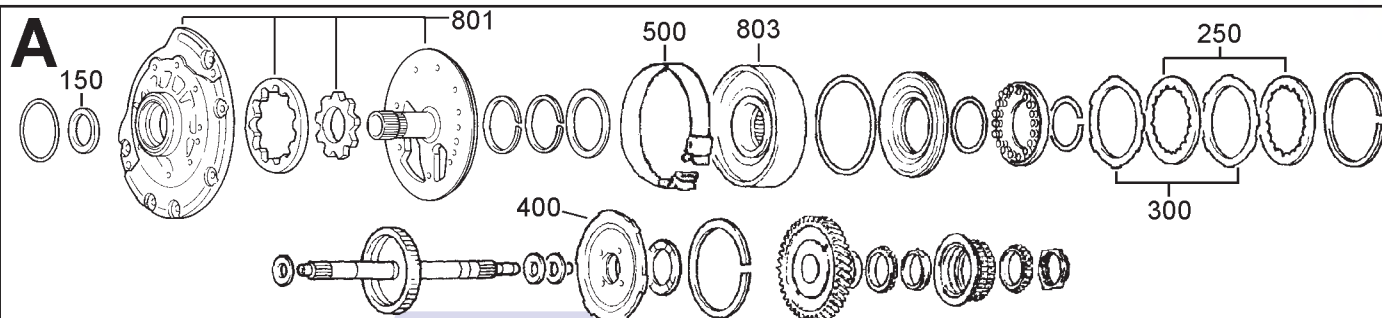
PUMP, REVERSE CLUTCH & INTERMEDIATE DRIVE GEAR
