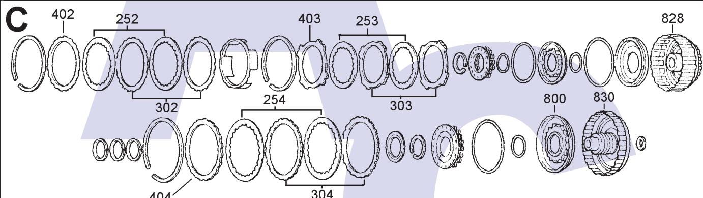
OVERDRIVE, COAST & FORWARD CLUTCHES
